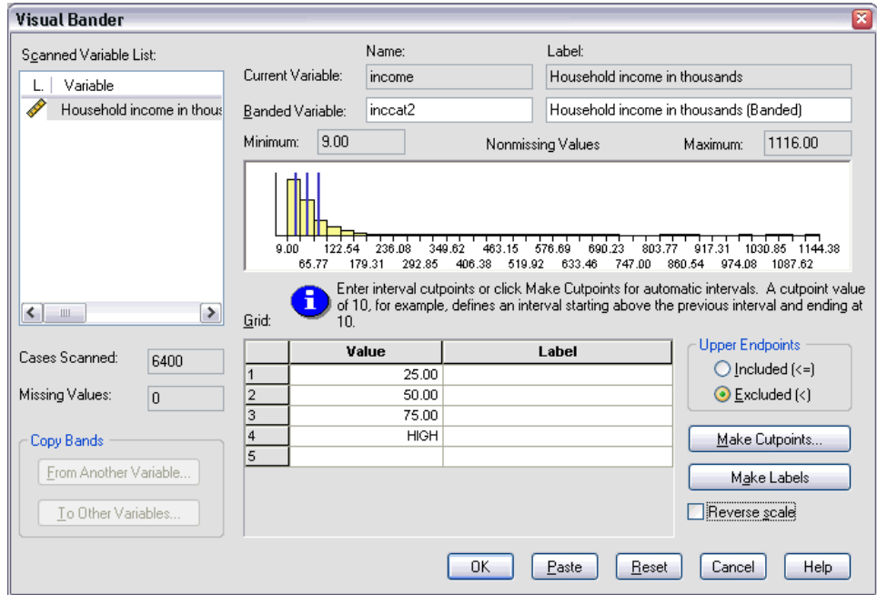
Figure 10-4 Main Visual Bander dialog box with defined cutpoints
